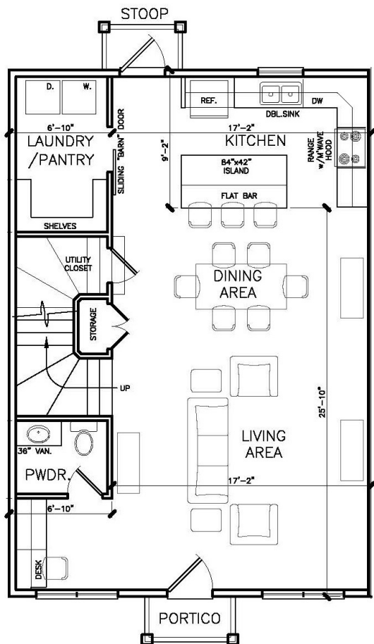
1st FLOOR PLAN PLAN 3A
