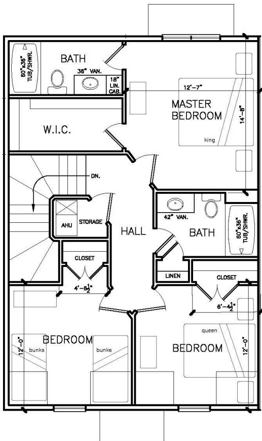
2nd FLOOR PLAN Plan 3A
